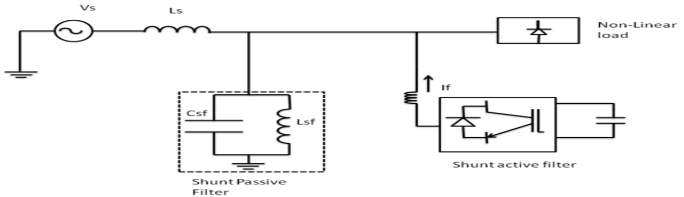
Fig.4.1: Block Diagram of Grid Feeding a Non-Linear Load with Shunt Passive Filter and Shunt Active Power Filter (SAPF) with Hysteresis Current Control (HCC).
