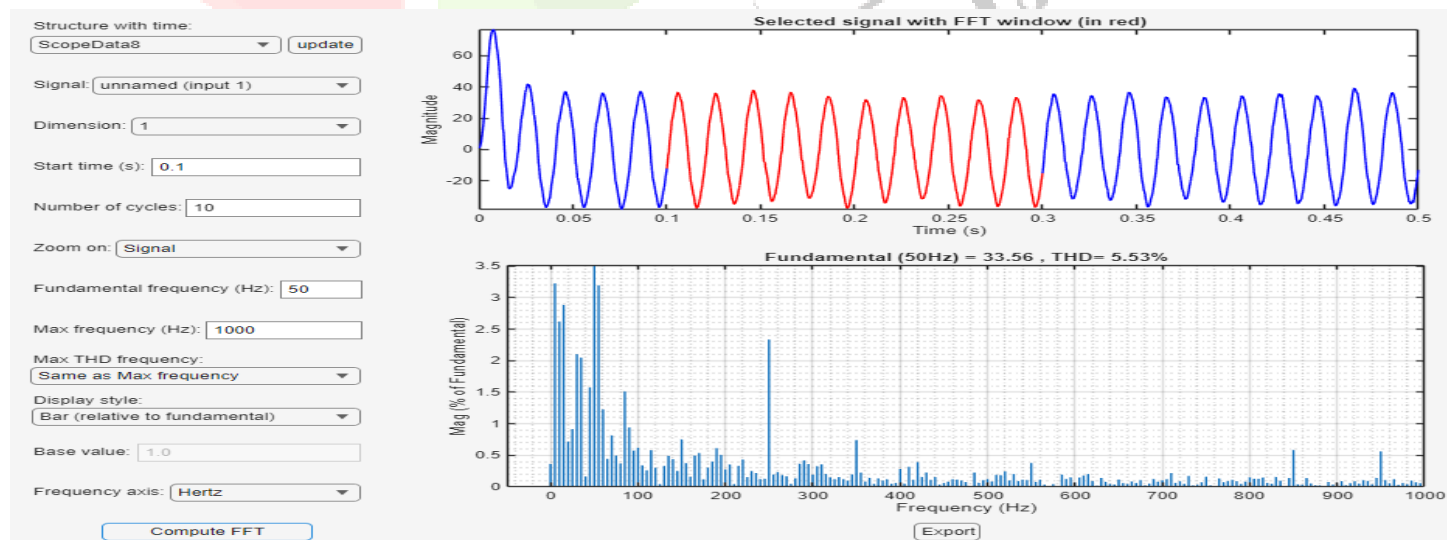
Fig :4.5 Harmonic spectrum of waveform
