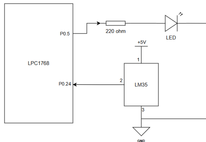
Figure 2: Circuit-level realization of the proposed ADC-driven edge inference system using the LPC1768 microcontroller, analog sensor interface, and GPIO-based alert output.
