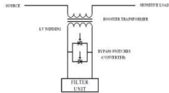
Fig 3 Standby mode
