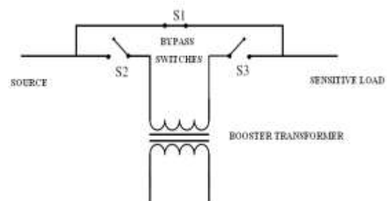
Fig 2: Protection mode
