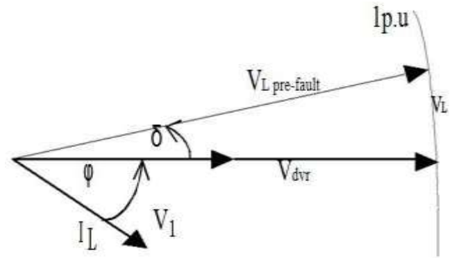
Fig.5. In-Phase compensation
