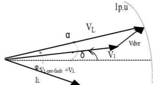
Fig.6. Phase advanced compensation
