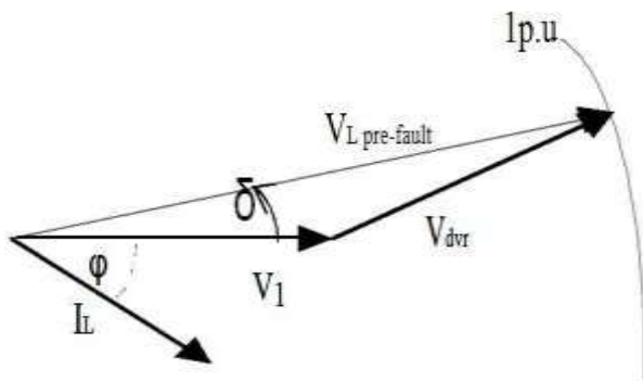
Fig.4. Pre-sag compensation
