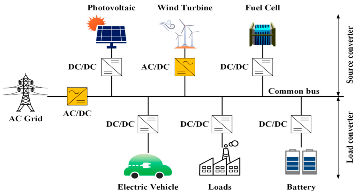
Figure.1:Schematic diagram of DC microgrid
