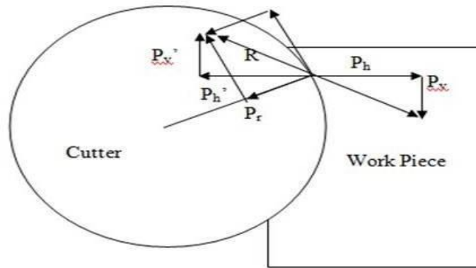
Fig. 2. Force Diagram
