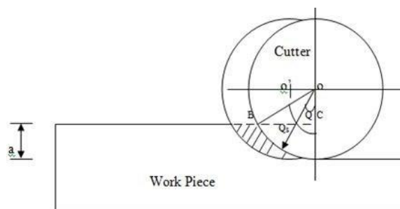
Fig. 3. Chip Cross Section
