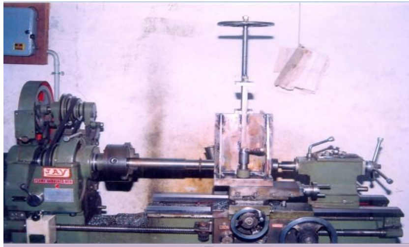
Fig. 7. Front view of the whole attachment
