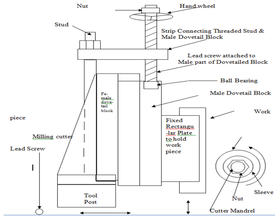
Fig. 5. Right side view of slotting and milling attachment to lathe
