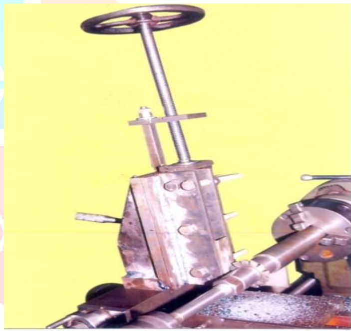
Fig. 8. Rear view of the whole attachment
