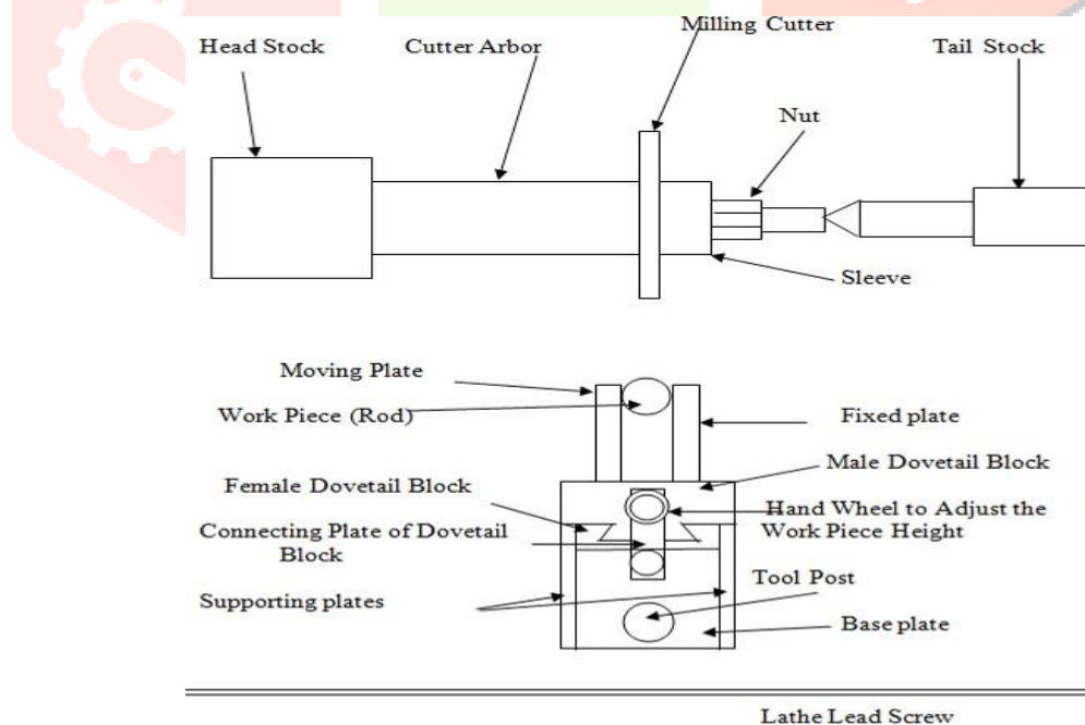
Fig. 4. Top view of slotting and milling attachment to lathe
